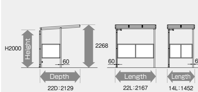
Single side panel type
