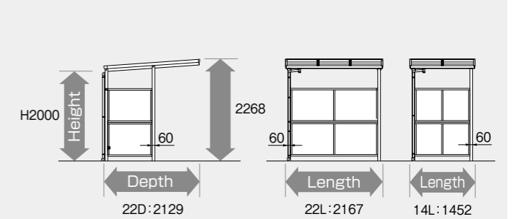
Double side panel type
